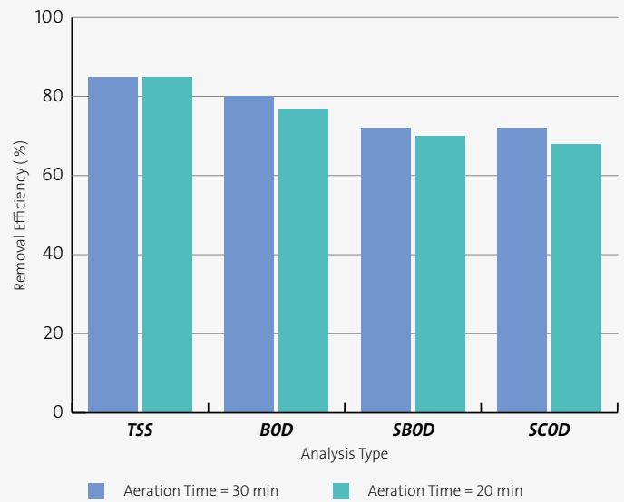
Pollutant reduction rates per aeration time (results obtained from pilot, Fort Smith STEP)
