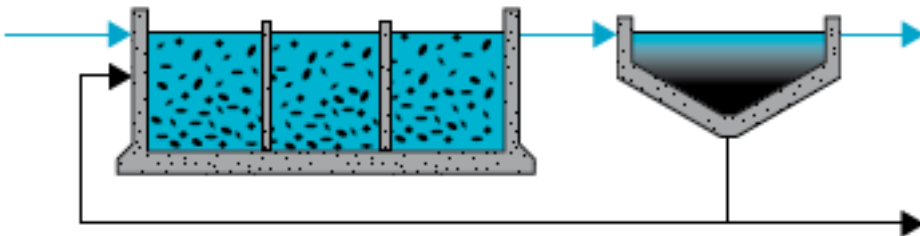
Hybas™ combination process with nitrification. Complete hybrid volume.
