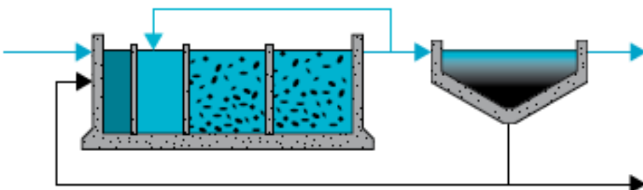
Hybas™ combination process with nitrification and pre-denitrification for nitrogen removal and selector for phosphorous removal.
