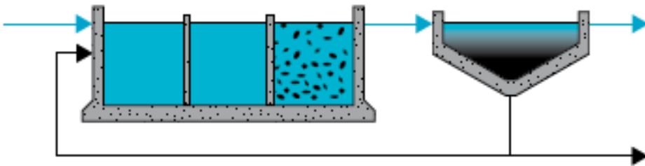
Hybas™ combination process with nitrification. Partial hybrid volume.
